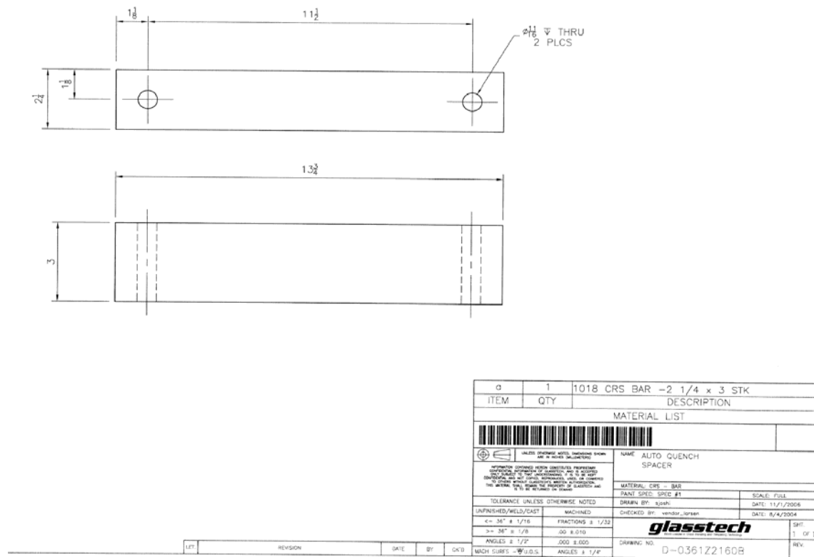
Spacer Block Detail Drawing (below- Qty. 2 Required)
