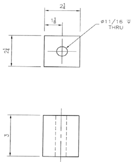
Spacer Block Detail Drawing (below- Qty. 2 Required)
